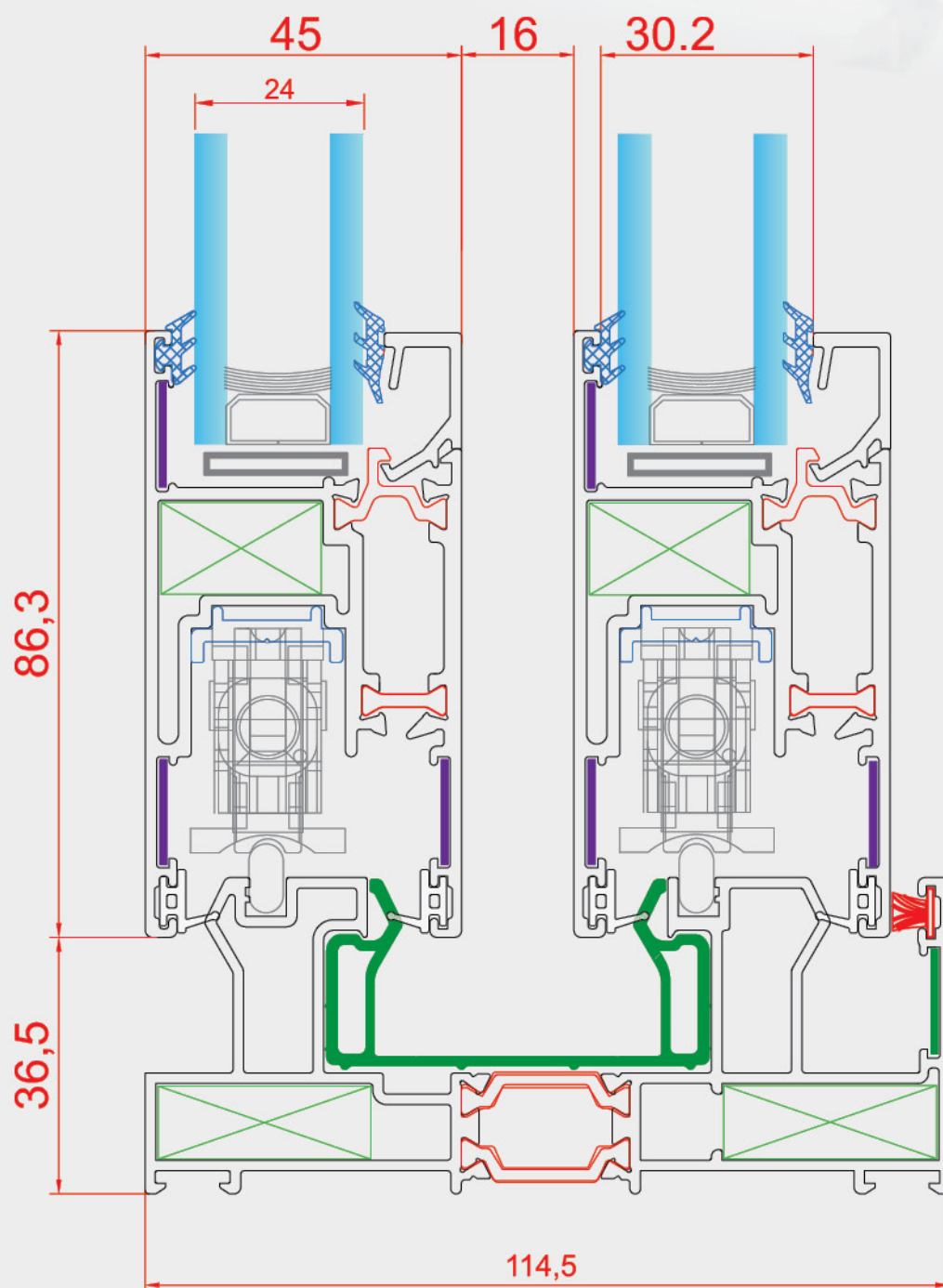
LIFT AND SLIDE 150 KG- GU 937
