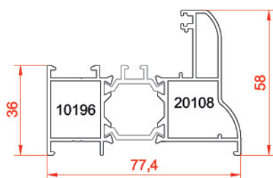
پروفیل کتیبه between two frame 10196-20108 weight: 1.399 kg/m
