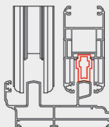
21073 Details Code: 53014
